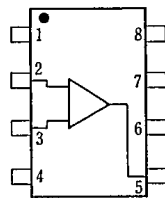
NJM386D NJM386M
