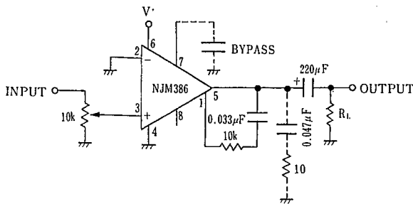
Amplifier 2
