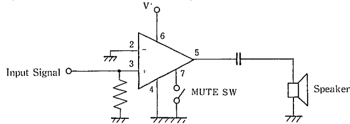
Amplifier 1
