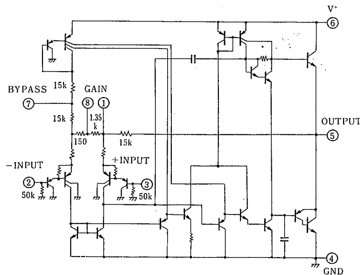
NJM386L
