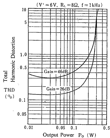
Total Harmonic Distortion vs. Output Power
